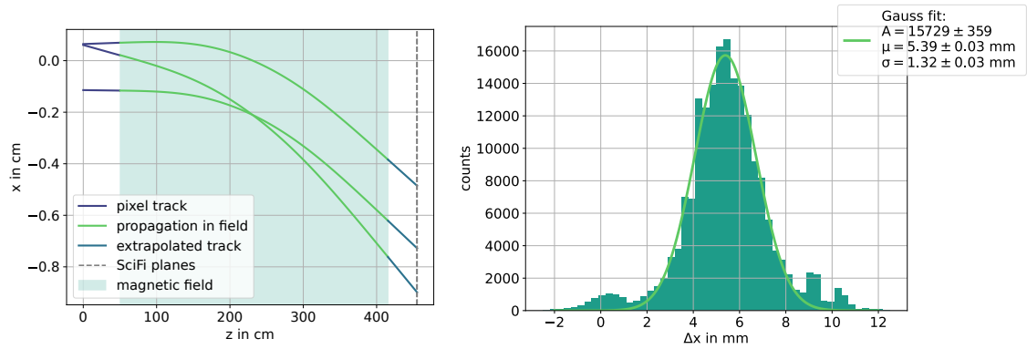
Figure 7.16: Track propagation through the GOLIATH magnetic field for three 400 GeV/ c proton tracks (left). Deflection in x of proton tracks at the first SciFi detector plane for an example run. The right-handed coordinate systems origin is the beam centre on the first pixel detector plane.
