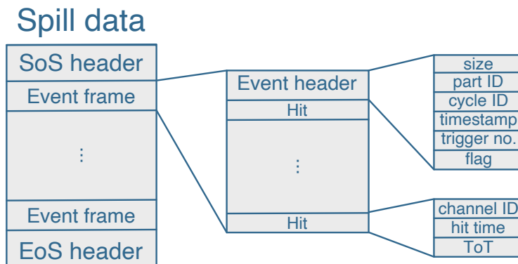
Figure 6.11: Visualisation of the data format sent to ControlHost. The data from one complete spill is sent after the EndSpill signal. The spill data frame consists of a header, followed by an individual frame for each event. The event frames begin with a dedicated header, containing information regarding the number of hits and unique event identification, followed by the registered hits. The hit data finally contains the unique channel ID, the timing relative to the trigger, and the ToT information.
