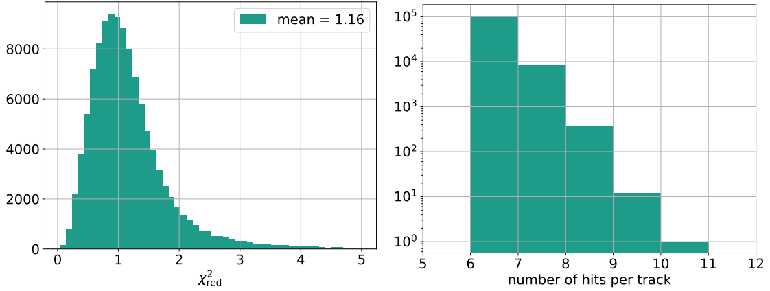
Figure 7.4: \chi^2/\text{ndf} distribution (left) and assigned clusters per track (right) for fitted tracks in physics CHARM 1 run 6. Pixel modules can overlap, such that tracks passing the overlapping regions can have more than six true clusters.
