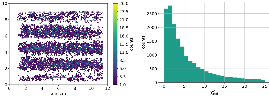
Figure 7.9: Position of matched tracks in the emulsion rest frame for CHARM 1 run 6 (left). The single spills can be clearly identified. \chi_{\text{red}}^2 distribution for matched tracks in the same run (right). The distribution peaks around 1.
