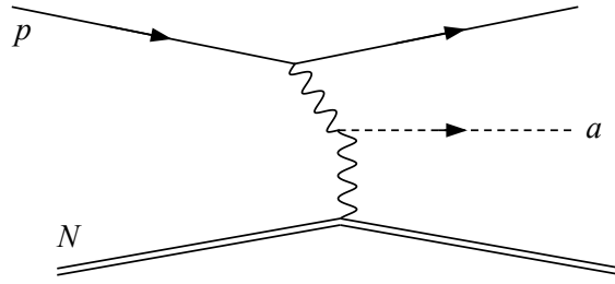
Figure 2.6: Primakoff production of an ALP in a beam-dump experiment. The incoming proton p scatters off a nucleus N . Two photons mediating the scattering process are converted to an axion with small transverse momentum. Adapted from [67, p. 6].
